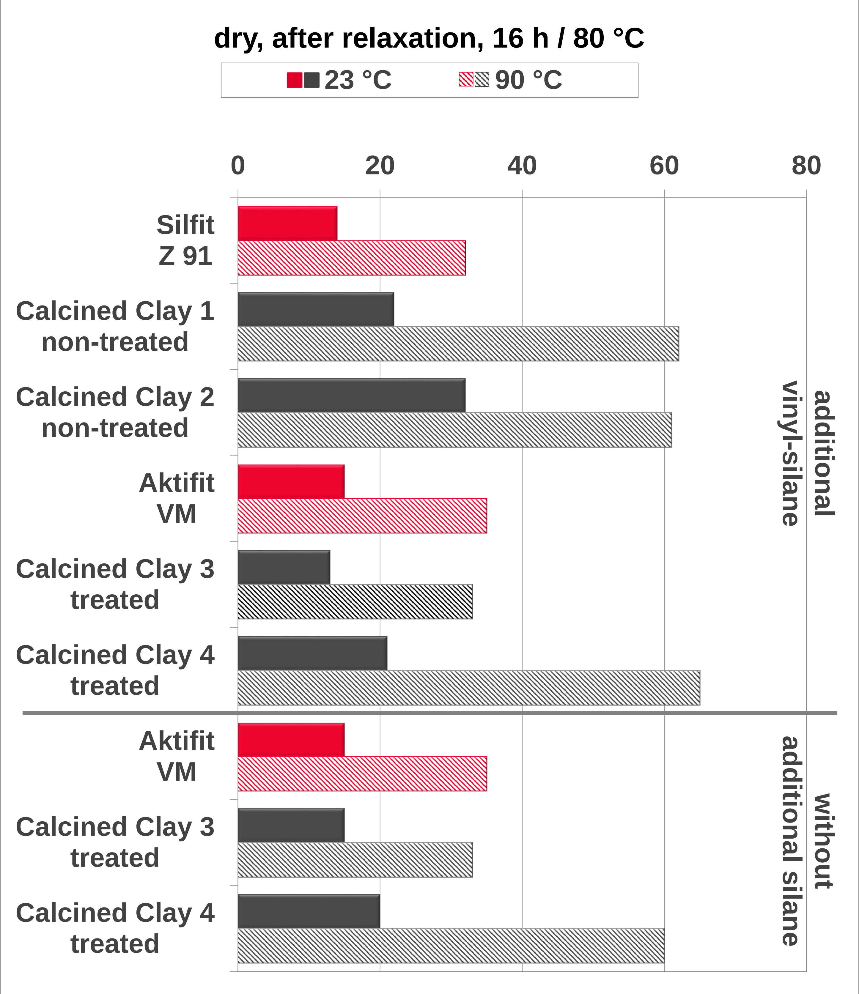
Dielectric Loss Factor \tan \delta , x 10 -4
